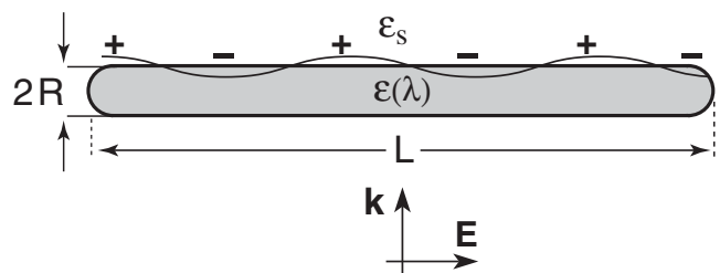
FIG. 1. A single antenna element represented by a metal rod. Incident light with wavelength \lambda polarizes the ends and gives rise to a standing surface charge wave.
