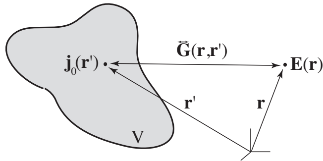
Figure 6.7: Illustration of the dyadic Green function \vec{\vec{G}}(\mathbf{r}, \mathbf{r}') . The Green function renders the electric field at the field point \mathbf{r} due to a single point source \mathbf{j}_0 at the source point \mathbf{r}' . Since the field at \mathbf{r} depends on the orientation of \mathbf{j} the Green function must account for all possible orientations in the form of a tensor.
