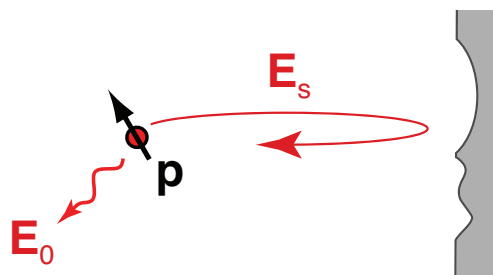
Figure 6.6: Illustration of dipole radiation in inhomogeneous environments. The total field is composed of a primary field \underline{\mathbf{E}}_0 directly radiated by the dipole and a secondary field \underline{\mathbf{E}}_s that is emitted by the dipole and then scattered at inhomogeneities in the environment.
