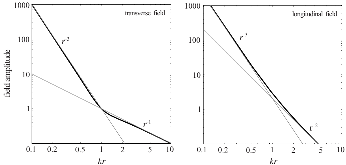
Figure 6.3: Radial decay of the dipole's transverse and longitudinal fields. The curves correspond to the absolute value of the expressions in brackets of Eqs. (6.44) and (6.45), respectively. While both the transverse and the longitudinal field contribute to the near-field, only the transverse field survives in the far-field. Notice that the intermediate-field with (kr)^{-2} does not really show up for the transverse field. Instead the near-field dominates for (kr) < 1 and the far-field for (kr) > 1 .
