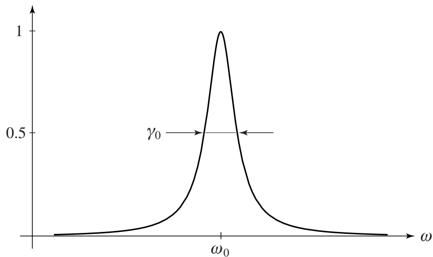
Figure 6.9: Lorentzian lineshape function as defined by the expression in brackets in Eq. (6.84).
