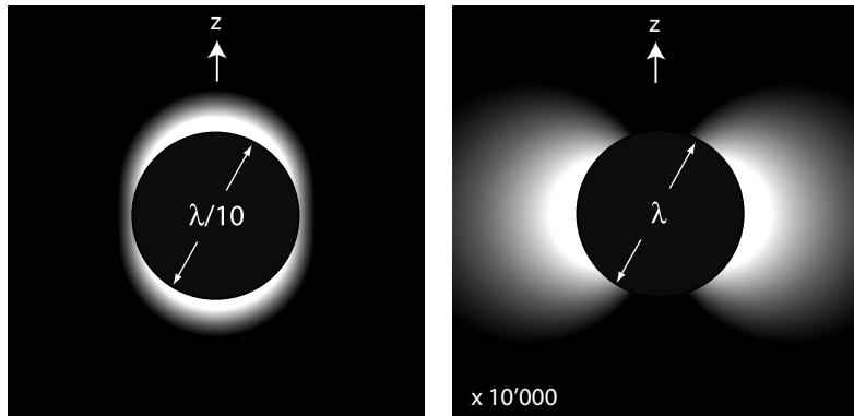
Figure 6.5: Electric energy density outside a fictitious sphere enclosing a dipole \mathbf{p} = p\mathbf{n}_z . (Left) Close to the dipole's origin the field distribution is elongated along the dipole axis (near-field). (Right) At larger distances the field spreads transversely to the dipole axis (far-field).
